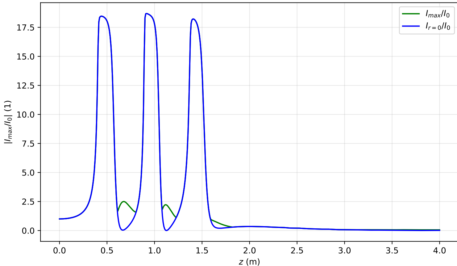
I_{max}(x = 0, y = 0, z)/I_0 , \text{Pin}=6.0\text{Pcr} , artificial time
